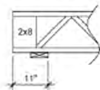
FIGURE 1—BEARING POSITION ALLOWED AND MAXIMUM FIELD CUT
